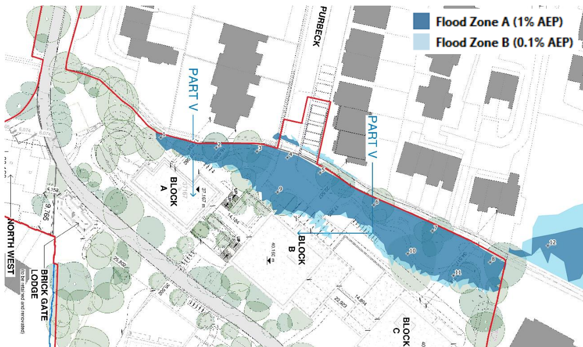
Figure 4.2: Proposed Development overlain with Flood Zones
