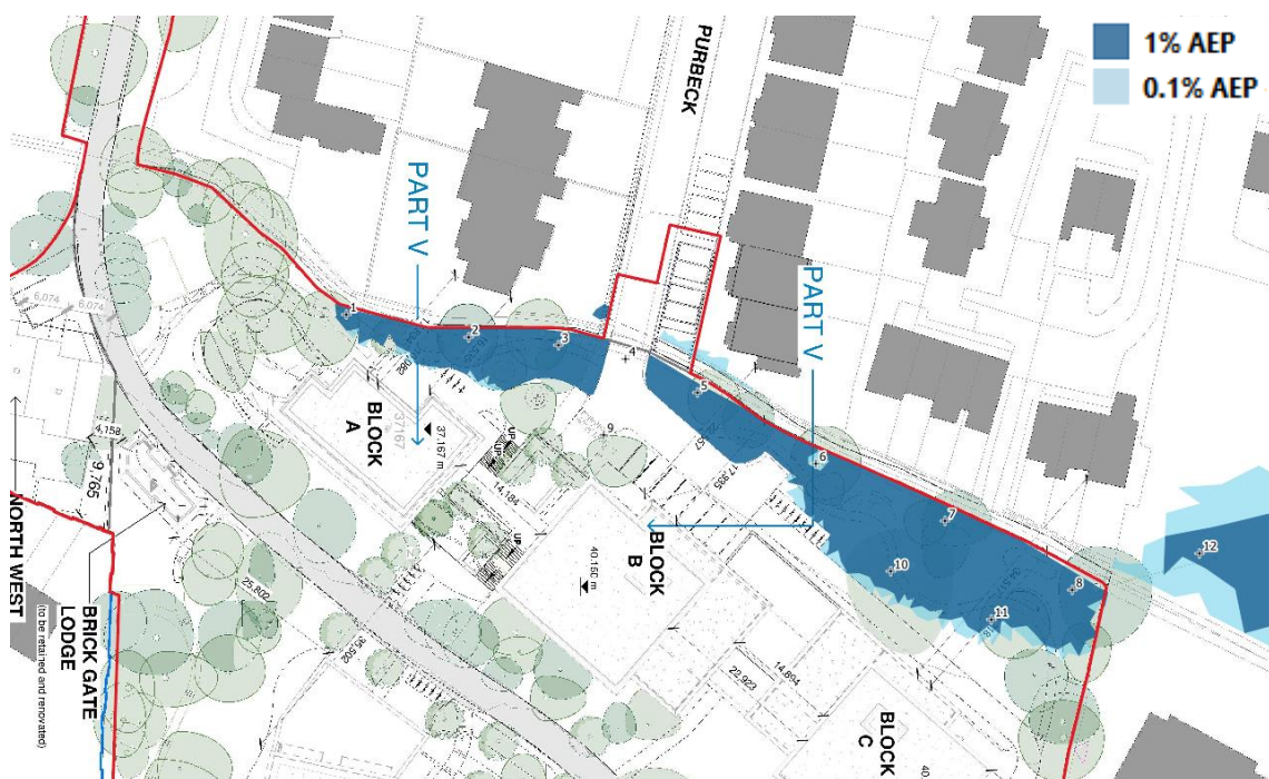
Figure 4.3: Proposed Scenario (Present Day) Flood Map
