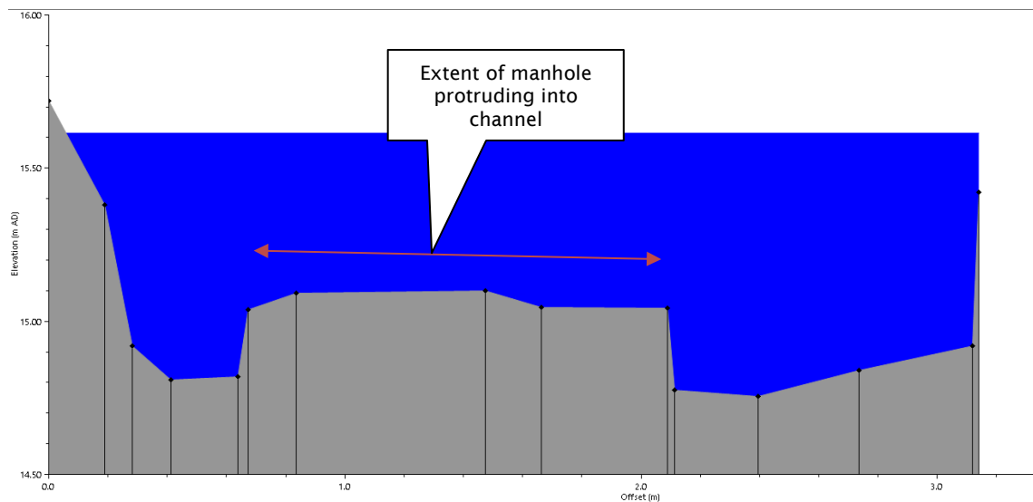
Figure C.4: Manhole Obstruction
