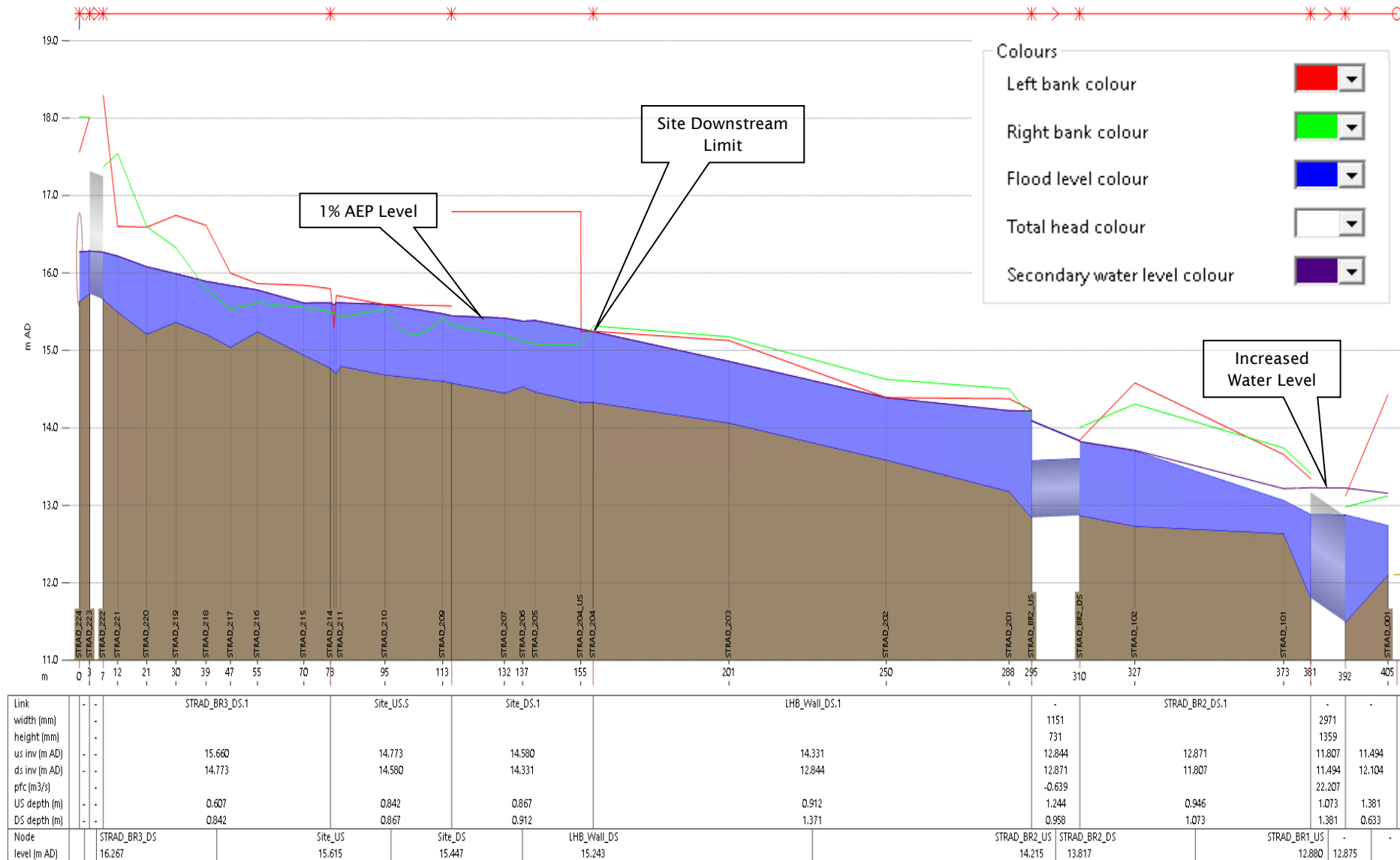
Figure C-7 Sensitivity Testing - Boundary
