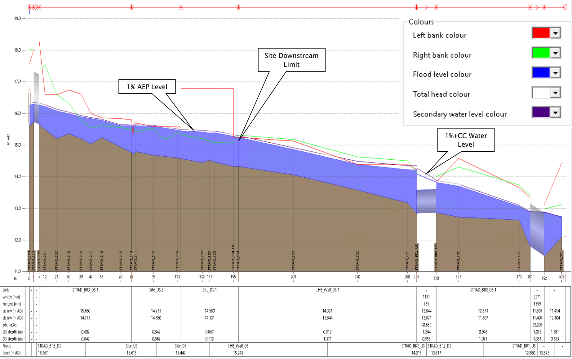
Figure C-6 Sensitivity Testing - Flow
