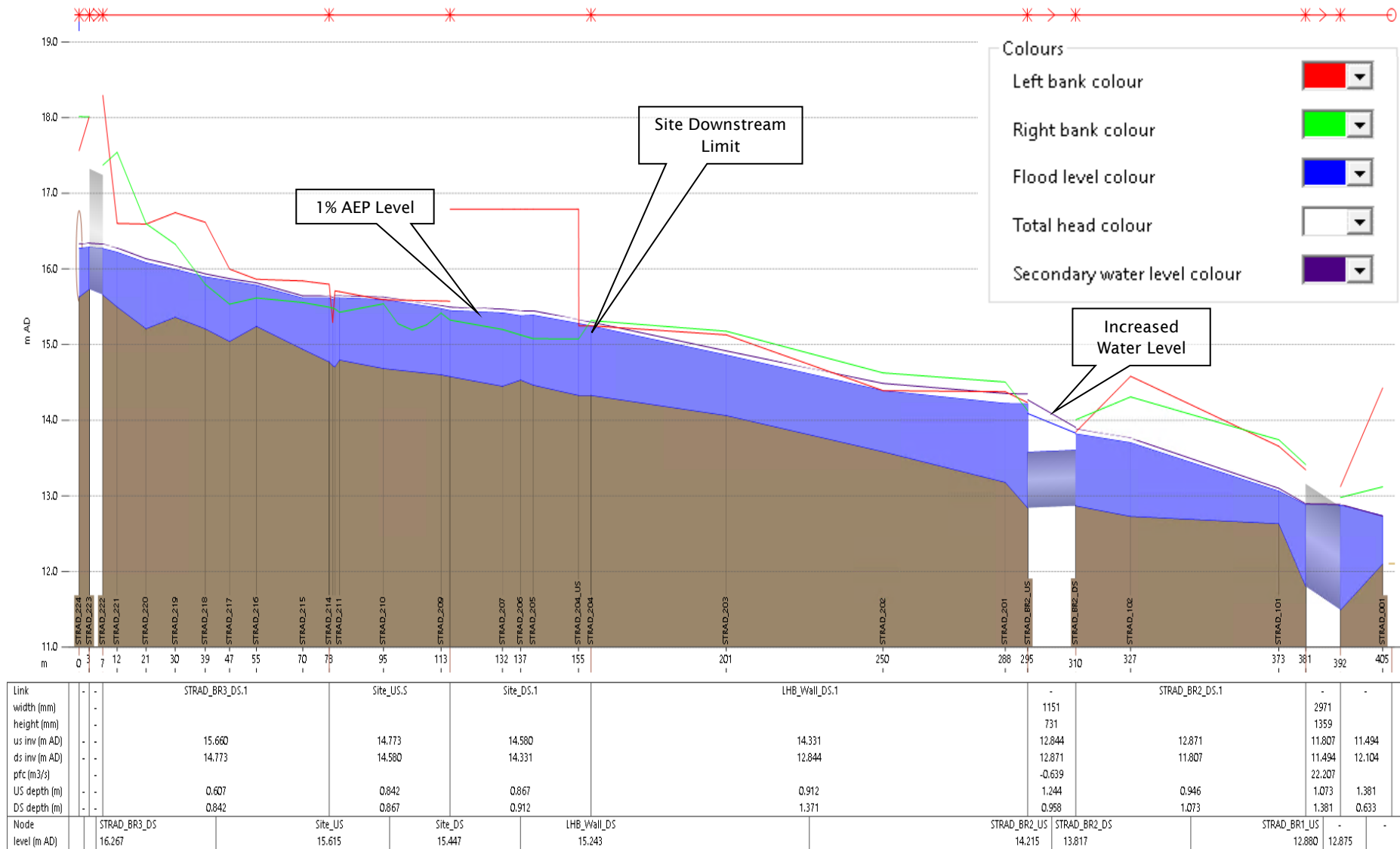
Figure C-5 Sensitivity Testing - Roughness
