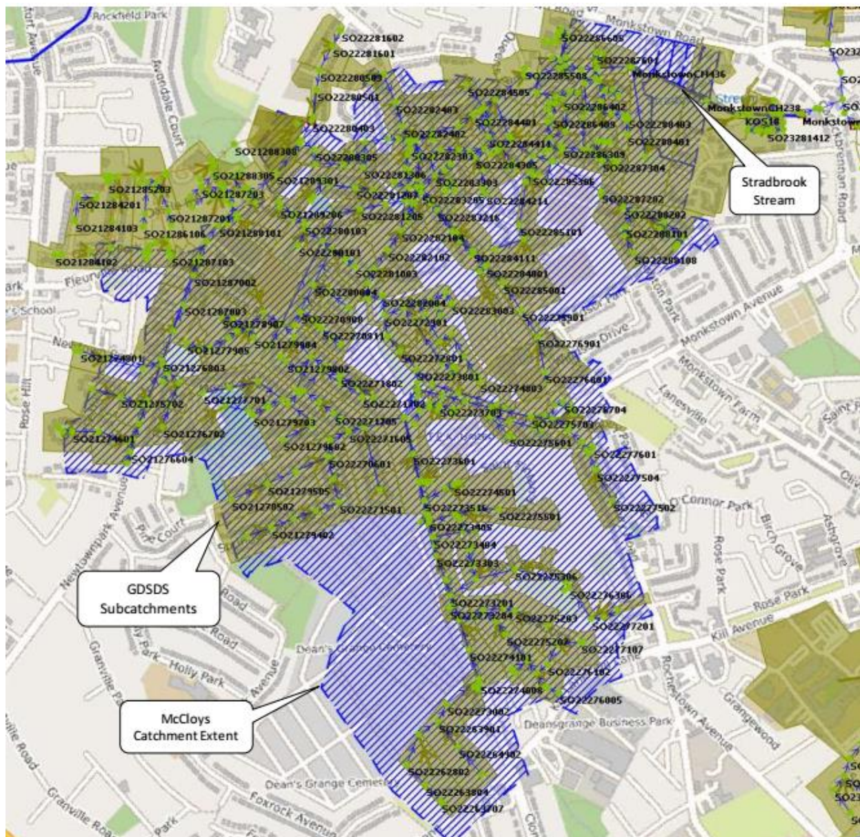
Figure C.1: GDSDS vs McCloy Catchment
