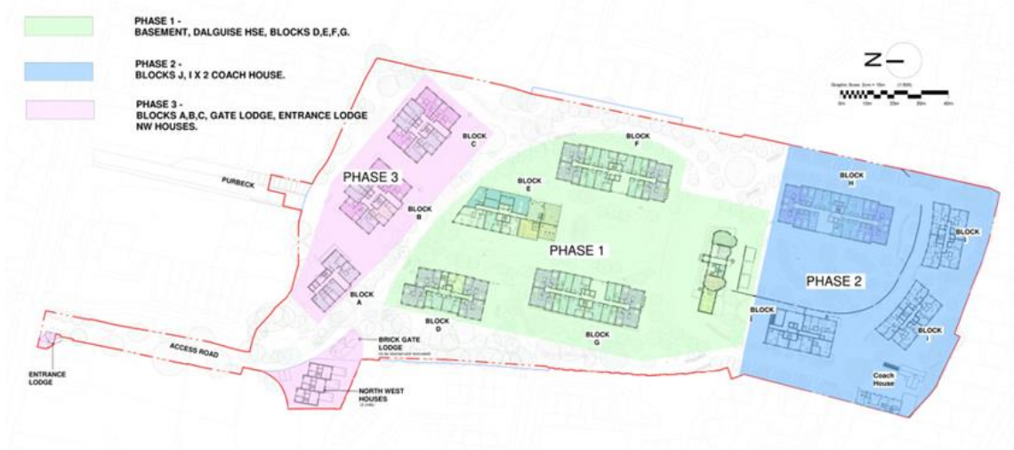
Figure 5.1: Illustrative Plan showing proposed construction phasing.
